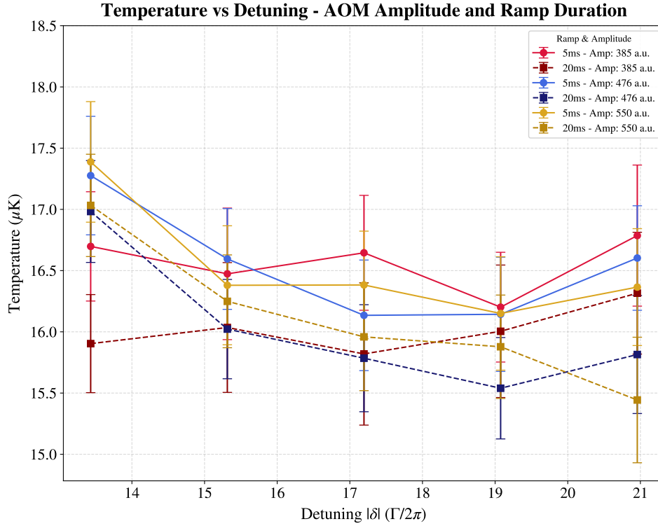
Figure 3.3: Optical molasses temperature versus cooling detuning for different AOM amplitude and ramp durations. No clear optimal AOM amplitude is observed as the variations remain within the uncertainty. Temperatures corresponding to a ramp duration of 20 ms (dashed lines) are systematically lower than those obtained with a 5 ms ramp (solid lines).
