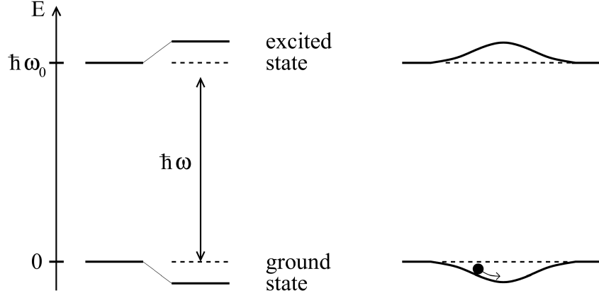
Figure 1.7: From [7]. Left: light-shifted energy levels for a two-level atom for a red detuning ( \Delta < 0 ). Right: a spatially inhomogeneous field produces a potential well that traps the atoms.
