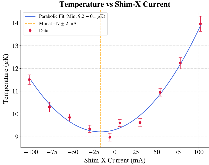
Figure 3.5: Optical molasses temperature versus Shim-X current. The parabolic fit yields a minimum temperature T = (9.2 \pm 0.1) \mu\text{K} at a current I_x = (-17 \pm 2) mA.
