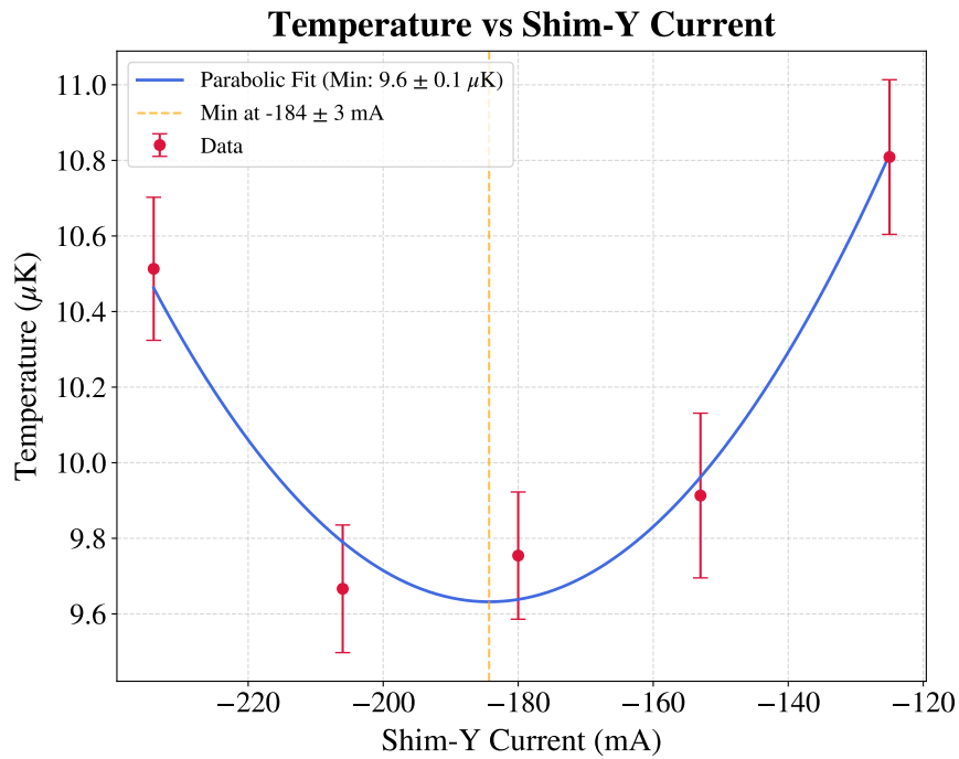
Figure 3.6: Optical molasses temperature versus Shim-Y current. The parabolic fit yields a minimum temperature of T = (9.6 \pm 0.1) \mu\text{K} at a current I_y = (-184 \pm 3) mA.
