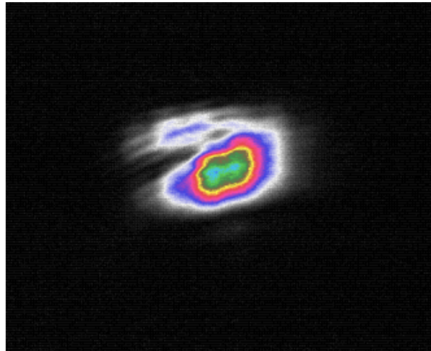
Figure 2.11: Final mode profile obtained after the injection optimization (magnification \sim \times 10 ). The mode shape is a bit deformed, meaning that it is a mixture of fundamental mode.
