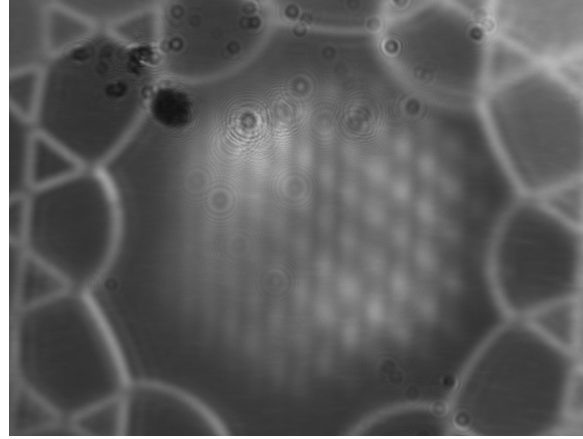
Figure 2.8: Images obtained with the FLIR camera using the microscope objective without the ocular lens. The mode clearly exhibits a hexagonal shape. Thanks to the FLIR high sensitivity and low read noise, the kagome structure remains visible even in this configuration. Artifacts in the top-left corner are dust grain deposited on the camera sensor.
