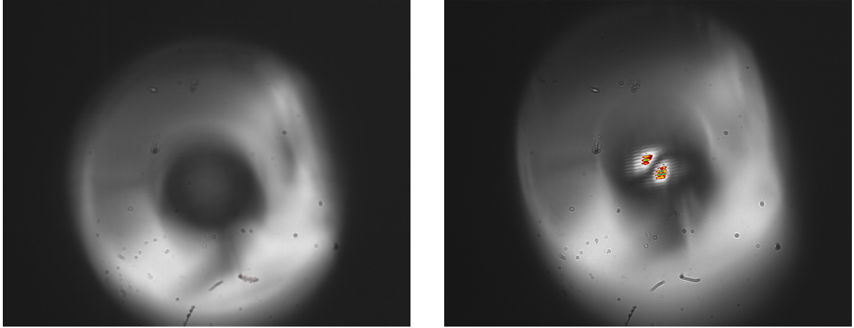
Figure 2.10: Preliminary images taken with a zoom \sim \times 10 of the fiber facet in the vacuum chamber (left) and the fiber with a non-optimized mode (right). In contrast to the test fiber images, here, the kagome structure is not illuminated, whereas the outer jacket is. The mode exhibits a clear LP_{11} profile. Note that focusing the mode bring the fiber out of focus, this makes the mode seem non-centered with respect to the fiber core.
