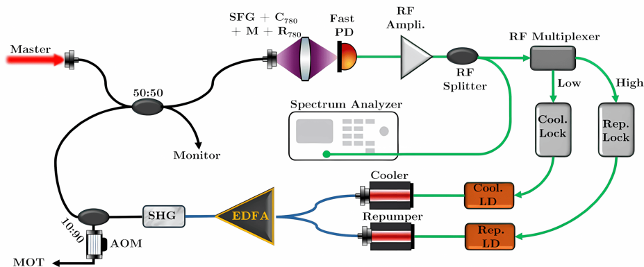
Figure 2.4: Cooling laser and repumping laser setup scheme.
