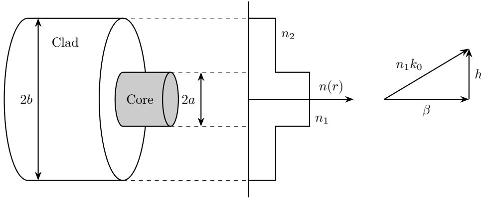
Figure 1.1: Schematic representation of a step-index optical fiber (left), and wave vector diagram showing the geometric relationship between the wave number in the core n_1 k_0 , the longitudinal propagation constant \beta , and the transverse wave number h (right).
