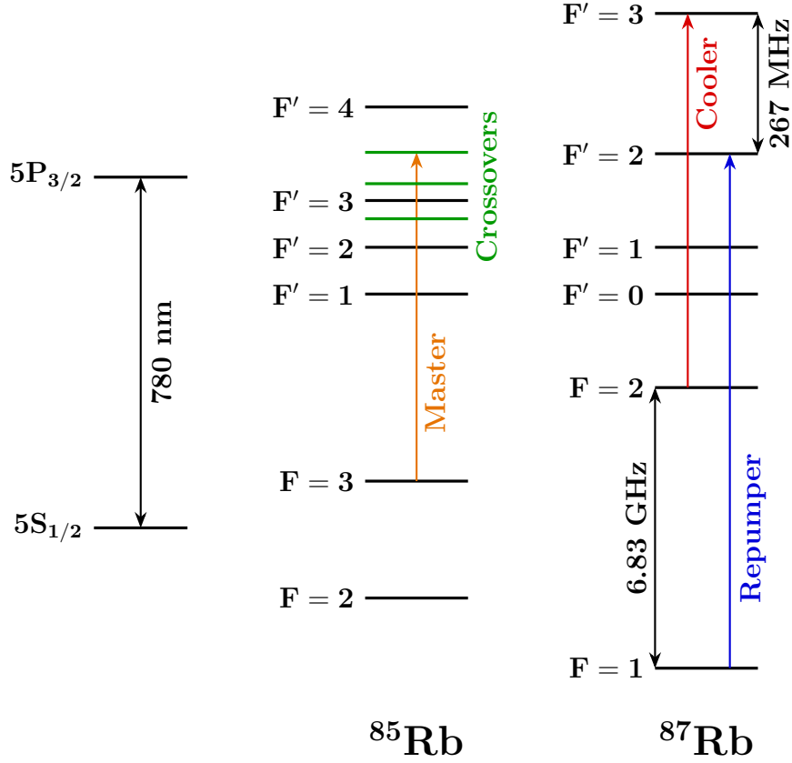
Figure 2.2: Level scheme of the ^{85}\text{Rb} and ^{87}\text{Rb} D_2 line. Reference transitions are indicated for the master laser (orange), cooler laser (red), and repumper laser (blue). For the ^{85}\text{Rb} also the crossover transition frequency of the saturation spectroscopy are drawn. Detailed data available in [11, 12].
