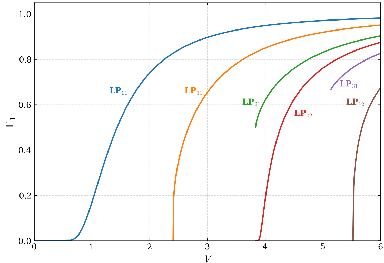
Core Confinement Factor \Gamma_1 of LP Modes
