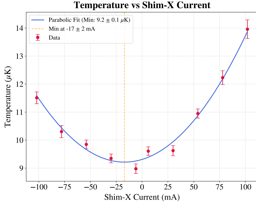
Figure 3.5: Optical molasses temperature Shim-X current. The parabolic fit retrieves a minimum temperature T = (9.2 \pm 0.1) \mu\text{K} at a current I_x = (-17 \pm 2) \text{ mA} .
