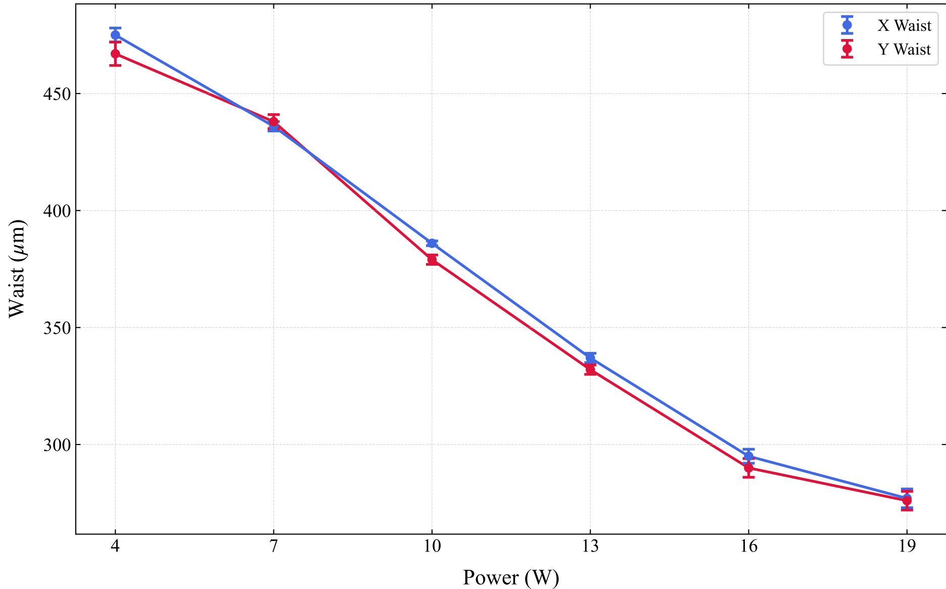
1064 nm Laser - Beam Waist vs Nominal Power (D4 \sigma - Gaussian fit mean)
