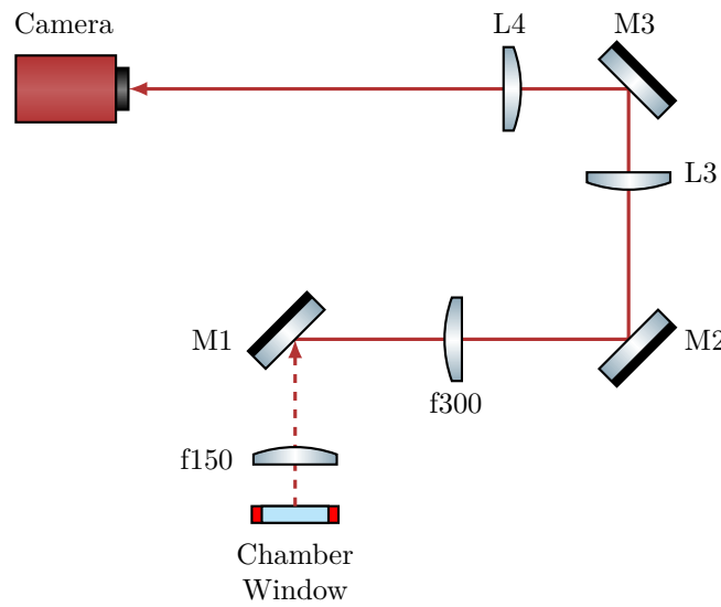
Figure 2.6: Scheme of the optical setup used to image the fiber inside the vacuum chamber. The optical path between the chamber window and the mirror M1 is vertical (characterized by the dashed beam line), whereas the rest of the setup is arranged horizontally on a breadboard mounted above the chamber. The focal length of lenses L3 and L4 were varied several times during the experiment. Most images were acquired using an f = 100 mm and an f = 500 mm providing an overall magnification of approximately \times 10 combined with the first imaging stage.
