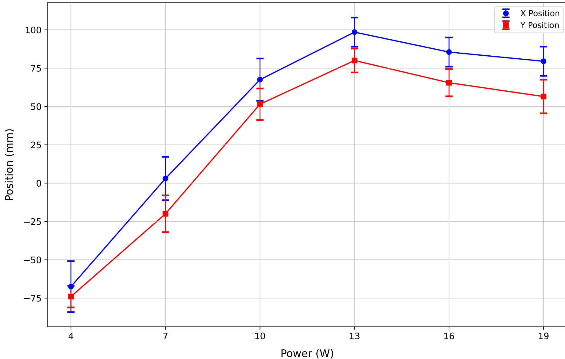
1064 nm Laser - Beam Waist Position vs Nominal Power (D4 \sigma - Gaussian fit mean)
