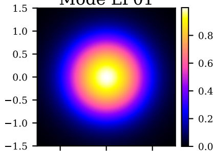
Mode LP01
