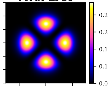
Mode LP21
