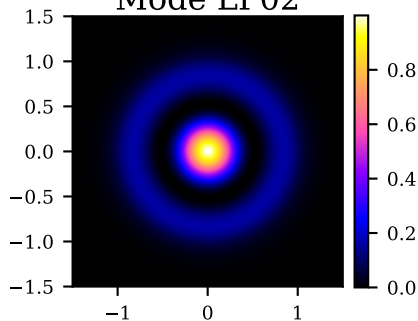
Mode LP02
