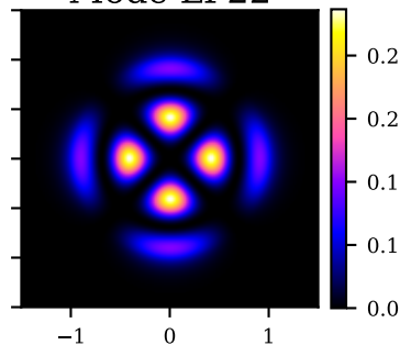
Mode LP22
