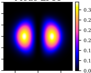
Mode LP11
