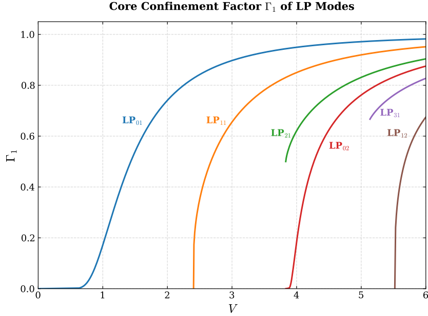
Figure 1.4: Confinement factor \Gamma_1 of LP modes as a function of the fiber V parameter. Not that for the modes with l > 1 ( LP_{21} , LP_{31} ) the confinement at cutoff is > 0 .
