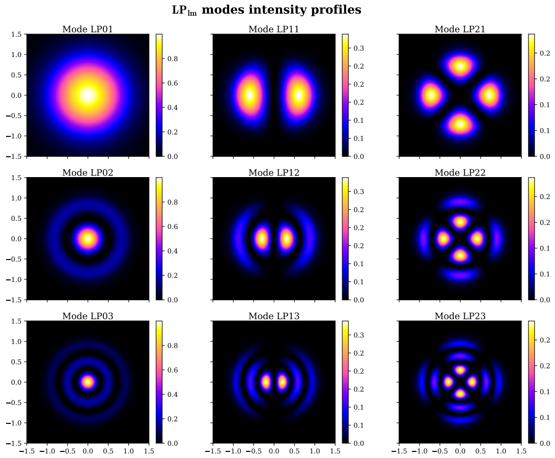
Figure 1.5: Intensity profiles of the LP mods with l = 0, 1, 2 and m = 1, 2, 3 . Each mode LP_{lm} is calculated with V^{(lm)} = V_{cutoff}^{(lm)} + 2 . The x, y coordinates are expressed in unit of the fiber core radius.
