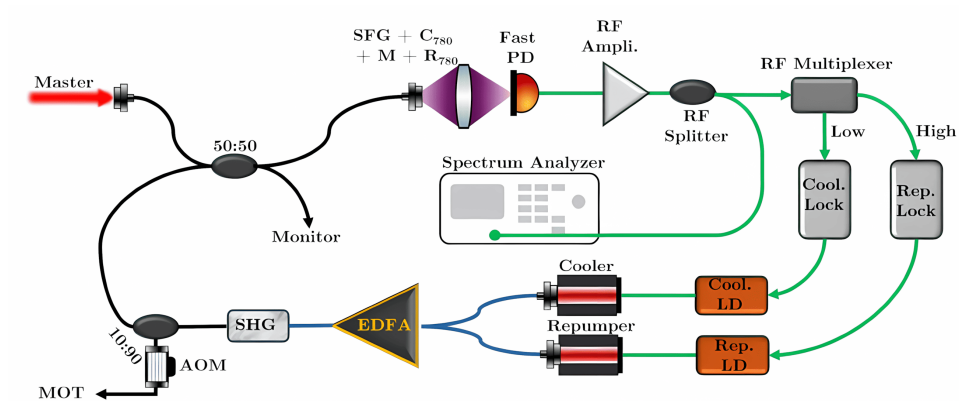
Figure 2.4: Cooling laser and repumping laser locking setup scheme.
