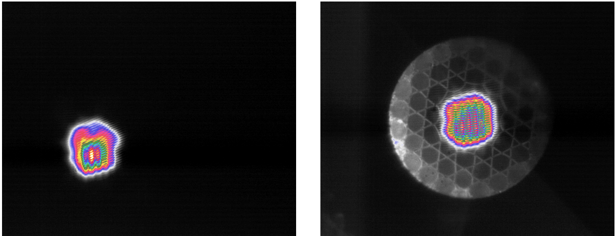
Figure 2.7: Images taken with the final horizontal microscope setup. Mode with \sim 80\% of transmission efficiency (left) and image of a mode with the kagome structure (right)
