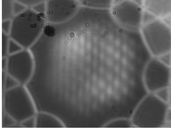
Figure 2.8: Image obtained with the FLIR camera using the microscope objective without the ocular lens. Notice that the mode shows a hexagonal shape. Thanks to the FLIR high sensitivity and low read noise, the kagome is visible also with this configuration without the ocular lens. The artifacts on the top left of the image are due to dust deposited on the sensor.
