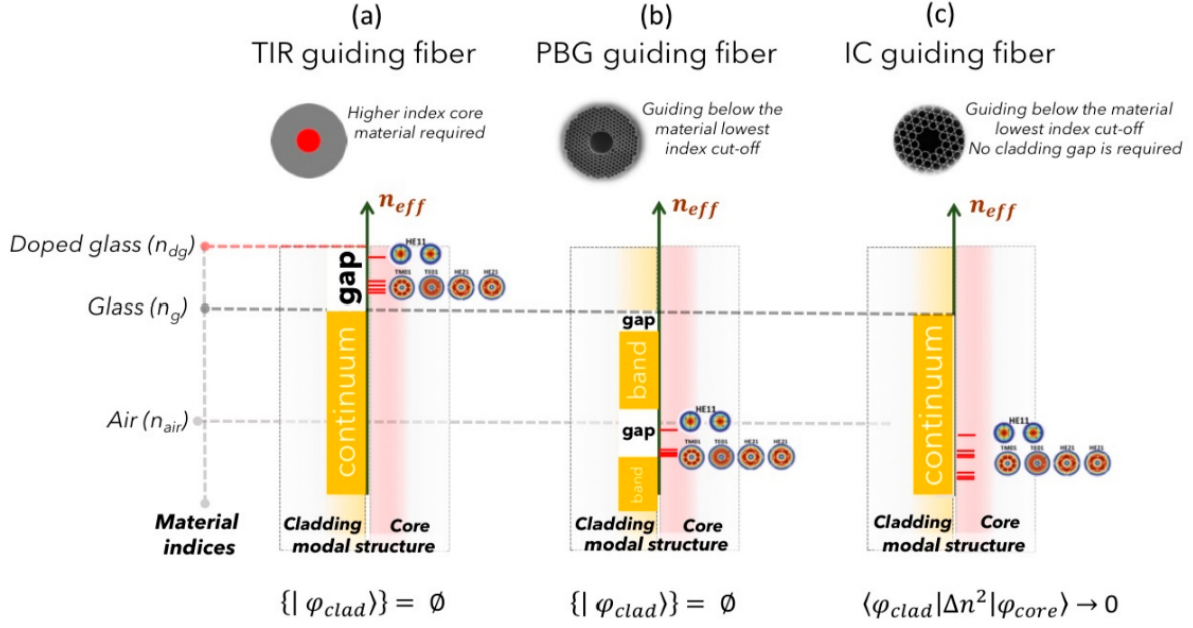
Figure 1.7: Modal content representation of optical guiding fibers: (a) Total internal reflection (TIR); (b) Photonic Band Gap (PBG); and (c) Inhibited Coupling (IC). The vertical axis represents the effective index n_{\text{eff}} , with the indices involved represented as horizontal dashed lines. Each graph represents the photonic bands of the cladding mode as a function of n_{\text{eff}} , with continuum (orange-filled rectangles) or gaps region (white-filled rectangles), highlighting where the core guidance happens. For both TIR and PBG fibers, the guided core modes appear in correspondence of gaps, whereas for IC fibers no gaps are present thus the guidance corresponds to the continuum of cladding modes. Credits [7].
