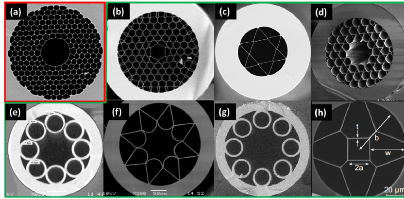
Figure 1.6: Scanning Electron Microscope images of some hollow core fibers: (a) photonic band gap fiber; (b-h) Inhibited Coupling fibers. Credits [8].
