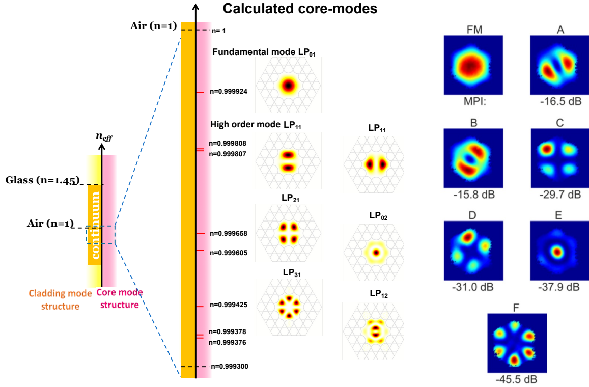
Figure 1.8: LP-like modes in HCPCFs. Left: effective refractive index spectrum and intensity profiles of the calculated LP modes for the core of a Kagome fiber. Credits [7]. Right: modal profiles experimentally measured via the S^2 technique on a 7-cell (K7) Kagome fiber, with the corresponding MPI. The image reports the fundamental mode (FM); two different orientation of LP_{11} -like modes (A, B); two different orientation of LP_{12} -like modes (C,D); an LP_{02} -like mode (E); and an LP_{31} -like mode (F). Credits [11].
