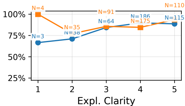
Under-reliance Mitigation Rate
