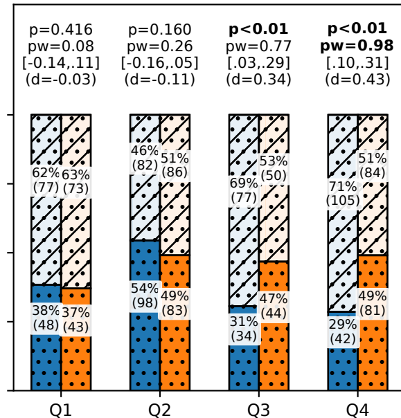
Expected: Reject
