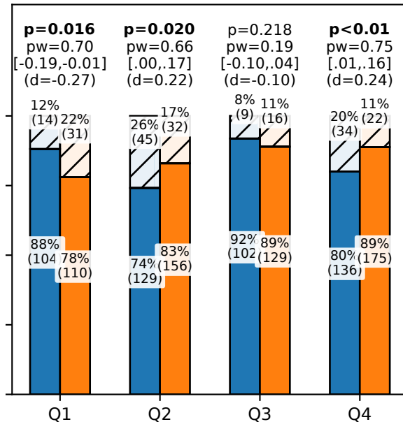
Expected: Accept
