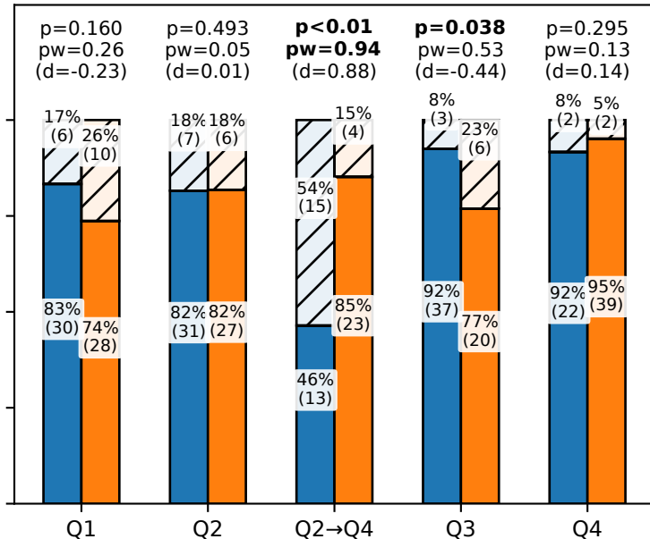
Expected: Accept
