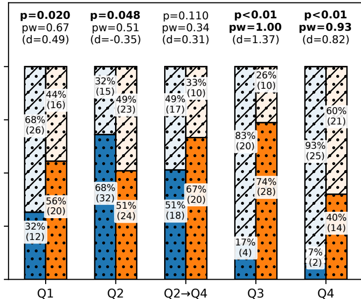
Expected: Reject
