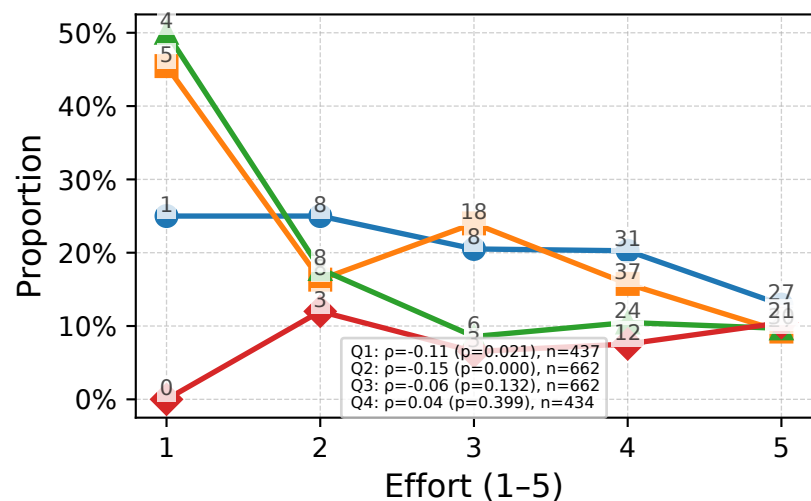
Under-reliance — Non-MAGIX
