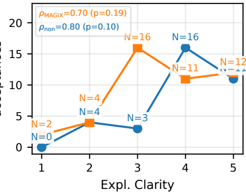
Appropriate acceptances
