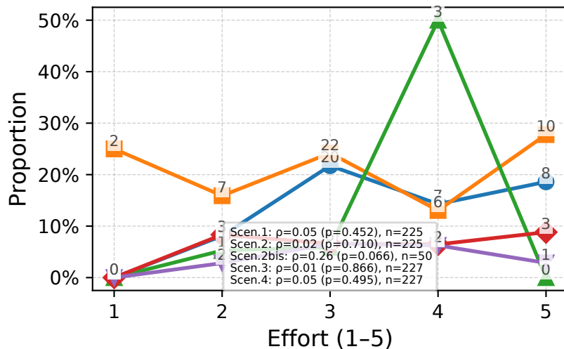
Under-reliance — Non-MAGIX
