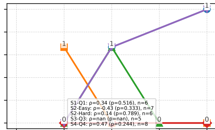
Under-reliance — MAGIX
