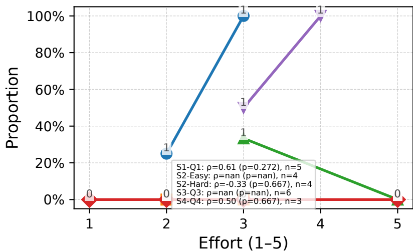
Under-reliance — Non-MAGIX
