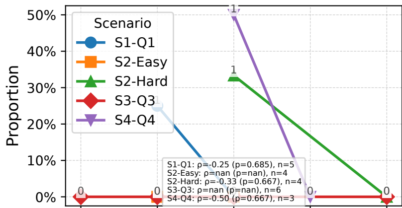
Under-reliance — Non-MAGIX
