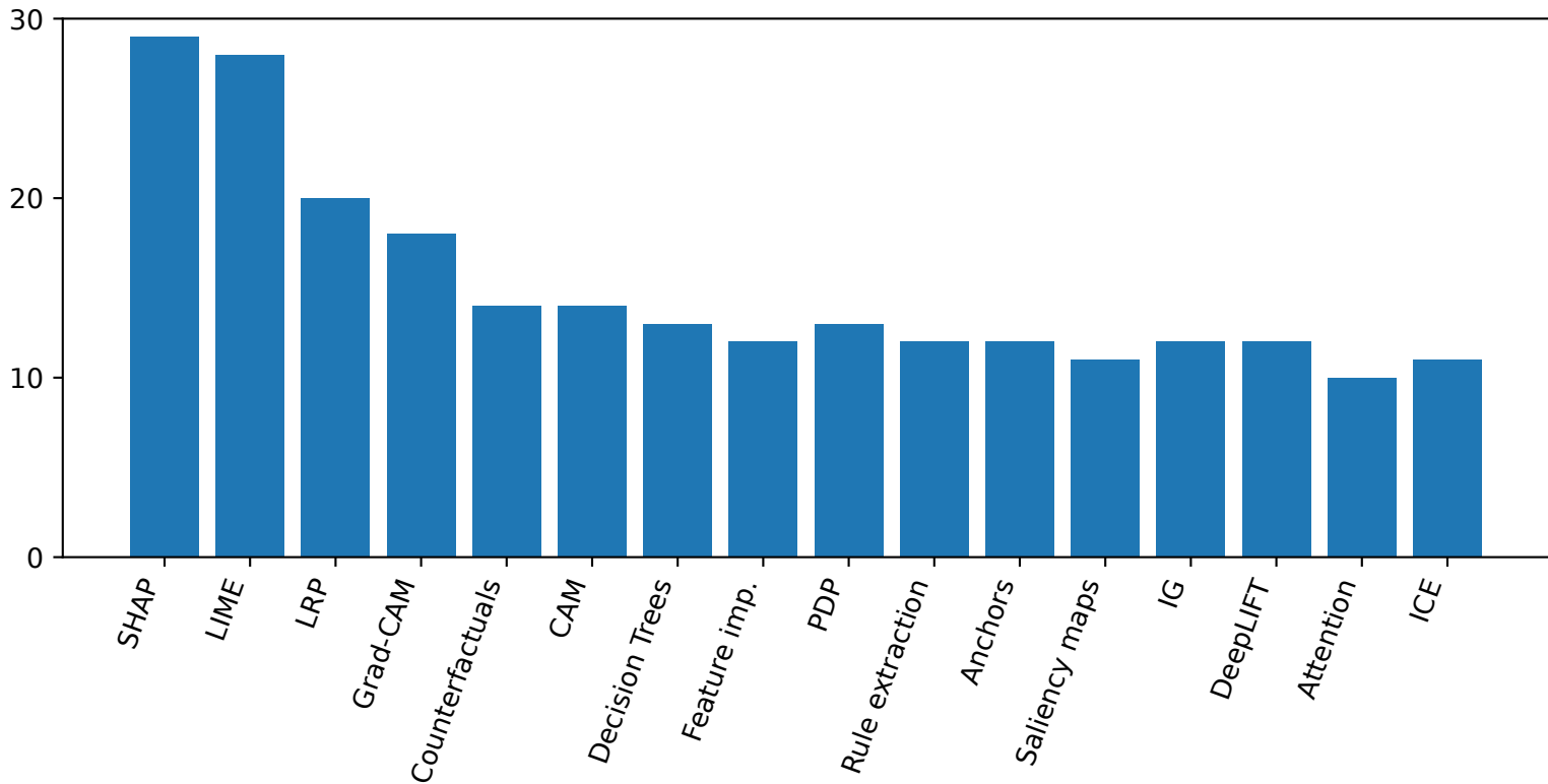
Survey mentions
