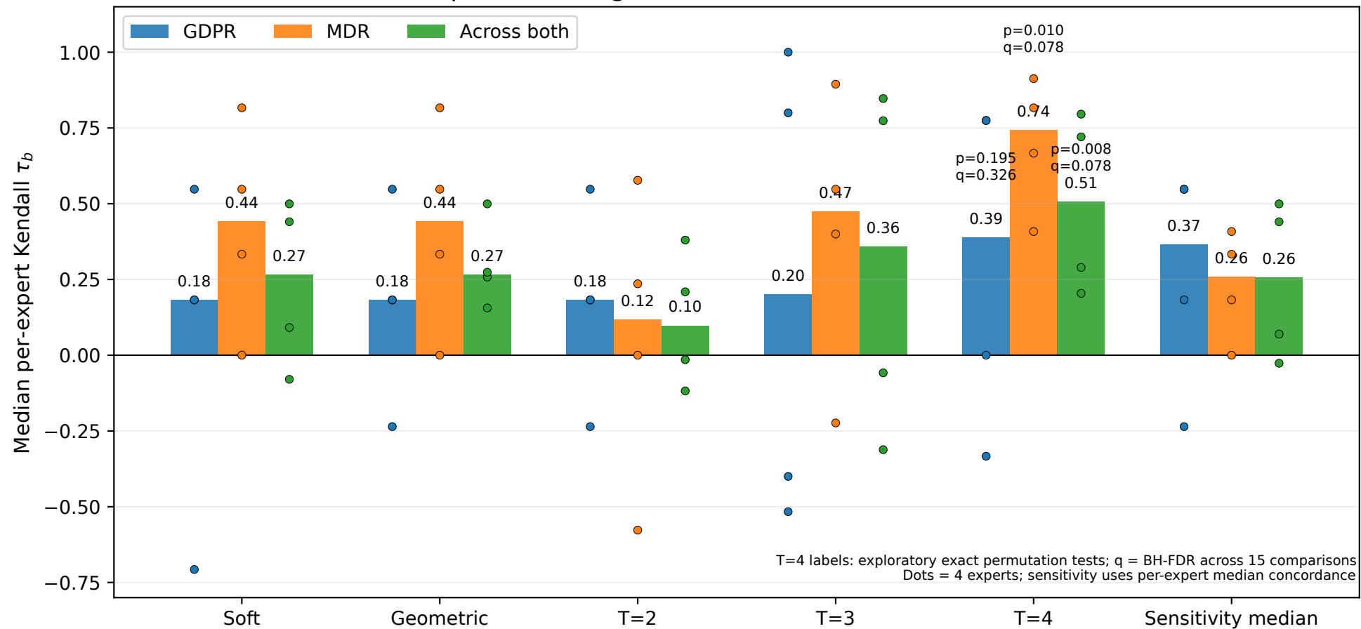
Formula-expert rank alignment across the two validation contexts
