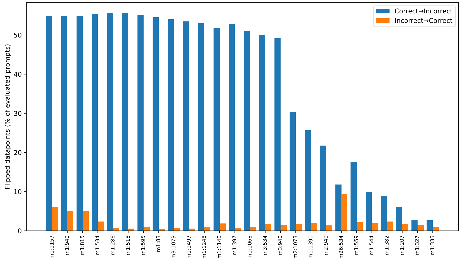
Top-26 neurons by flip rate (c2i vs i2c)
