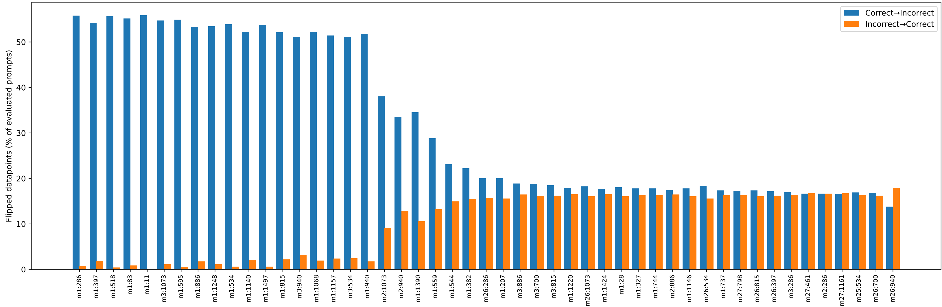
Top-49 neurons by flip rate (c2i vs i2c)
