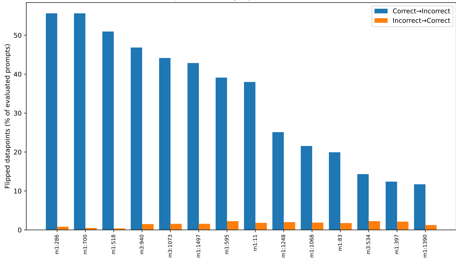
Top-14 neurons by flip rate (c2i vs i2c)
