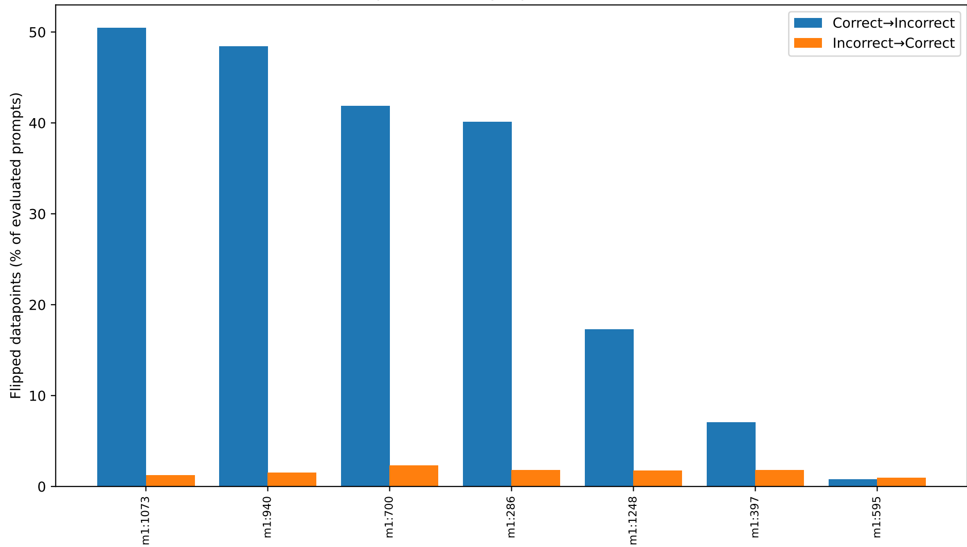
Top-7 neurons by flip rate (c2i vs i2c)
