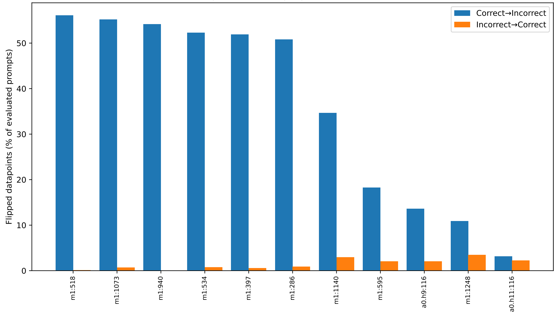
Top-11 neurons by flip rate (c2i vs i2c)
