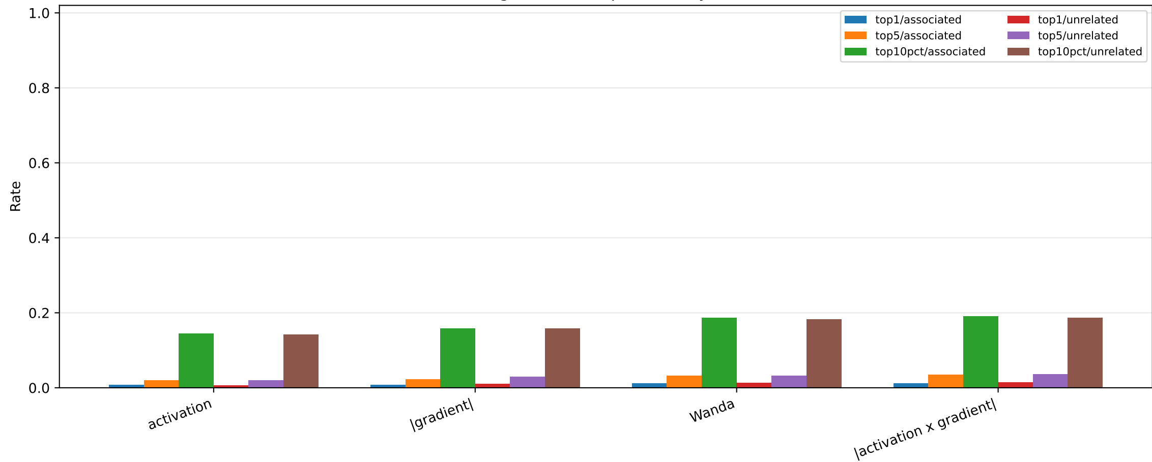
How often agonists are top-ranked by each metric
