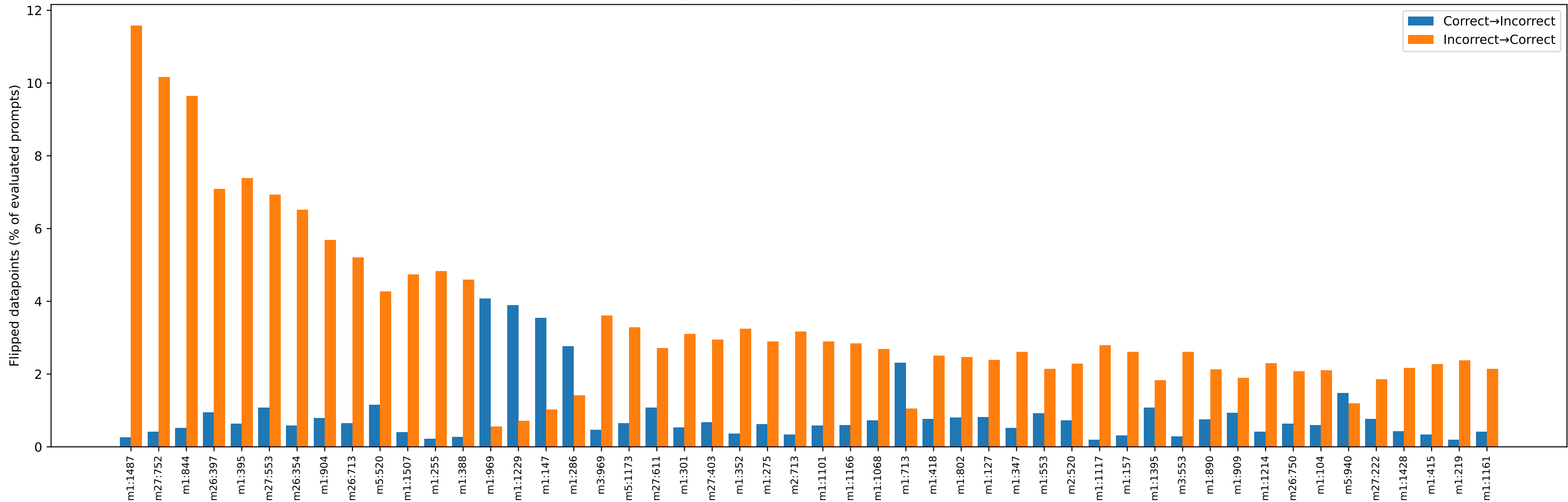
Top-50 neurons by flip rate (c2i vs i2c)
