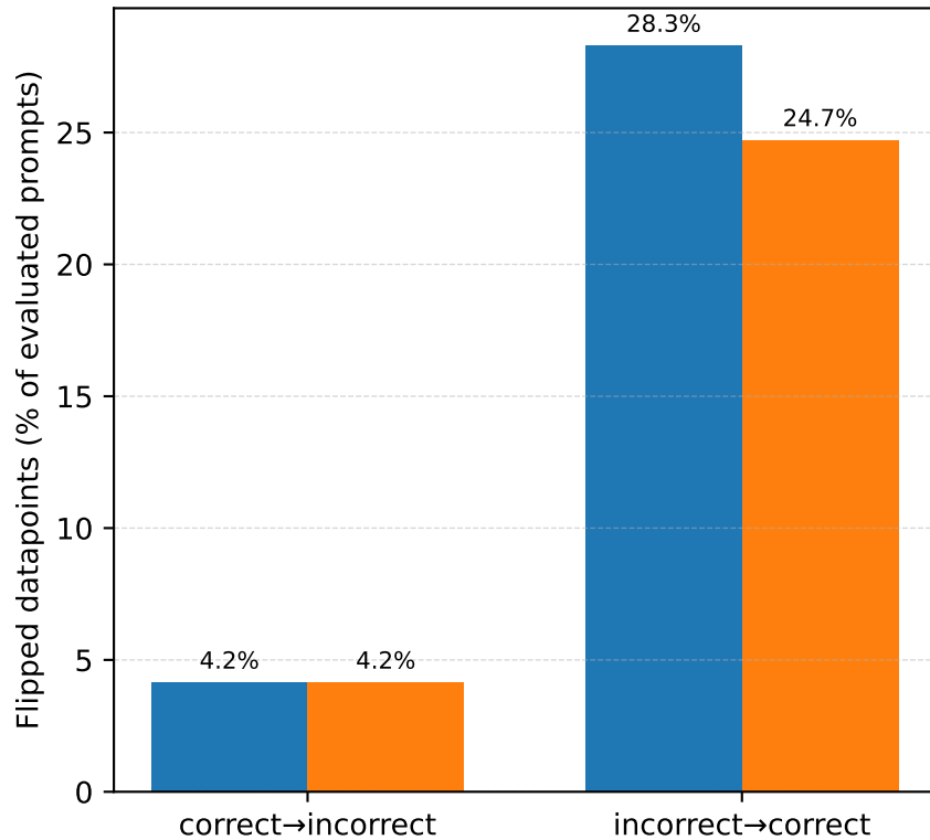
Unique flips explained by high-quality neurons (MCC \geq 0.85 )
