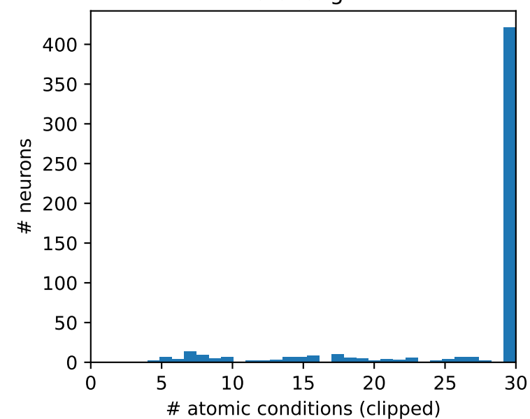
Rule length
