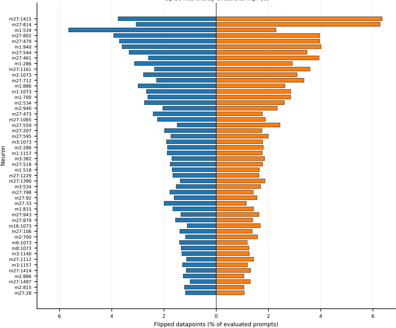
Correct→Incorrect Incorrect→Correct Top-50 neurons by directional flip rate
