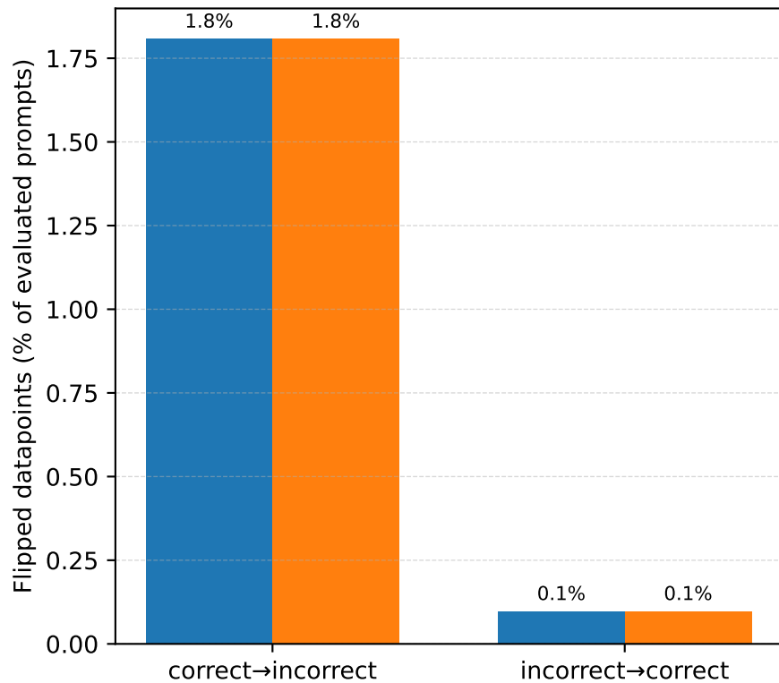
Unique flips explained by high-quality neurons (MCC \geq 0.85 )
