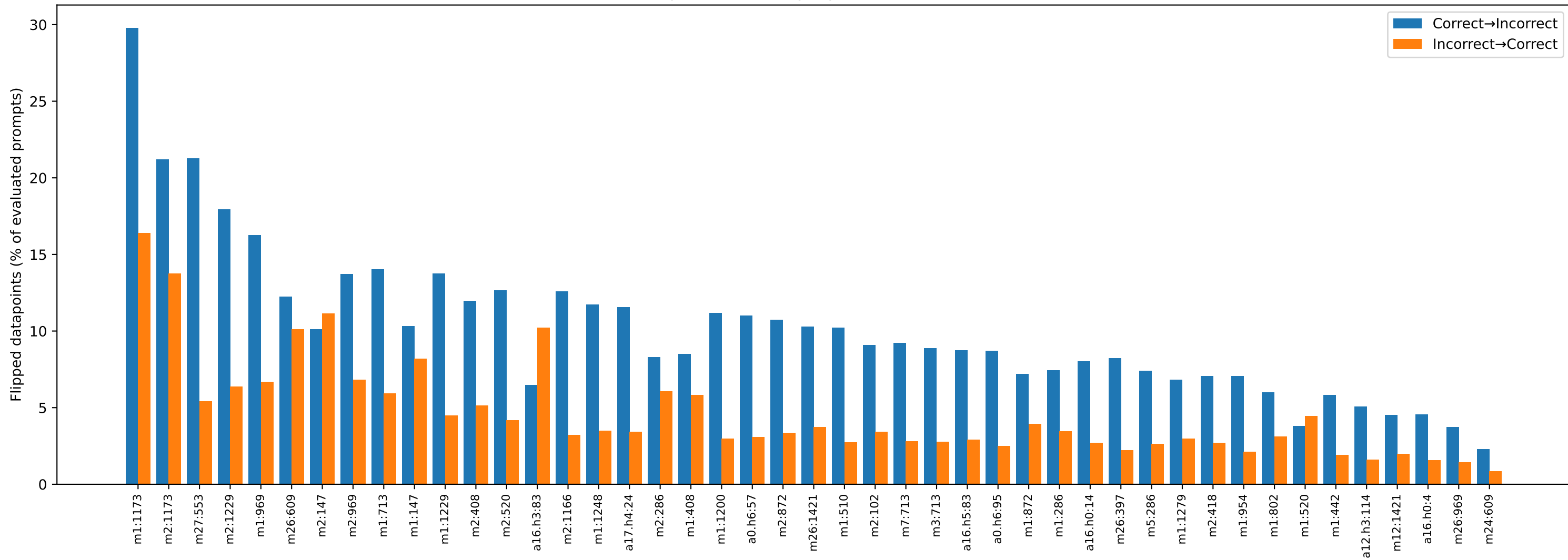
Top-45 neurons by flip rate (c2i vs i2c)
