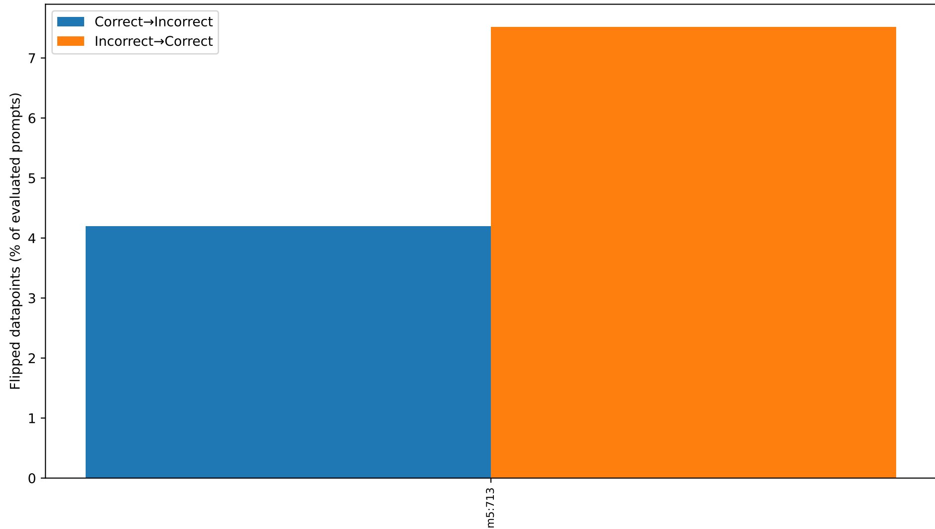
Top-1 neurons by flip rate (c2i vs i2c)
