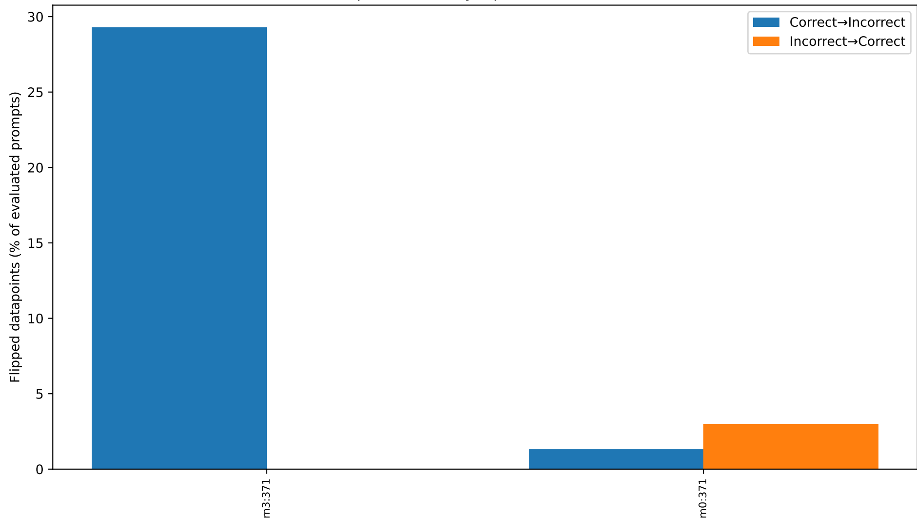
Top-2 neurons by flip rate (c2i vs i2c)
