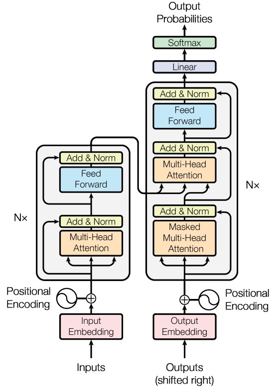
Figure 71: Architettura del Transformer: encoder (sinistra) e decoder (destra) impilati N \times , con multi-head attention, feed-forward, connessioni residue (Add & Norm) e positional encoding. Fonte: Vaswani et al., Attention Is All You Need (arXiv:1706.03762).
