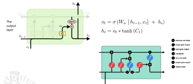
Figure 63: Output gate della LSTM: \mathbf{o}_t = \sigma(\mathbf{W}_o[\mathbf{h}_{t-1}, \mathbf{x}_t] + \mathbf{b}_o) e stato nascosto \mathbf{h}_t = \mathbf{o}_t \odot \tanh(\mathbf{C}_t) .
