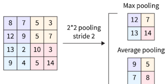
Figure 67: Max pooling e Average pooling a confronto.
