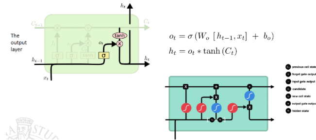
Figure 64: Output gate della LSTM: \mathbf{o}_t = \sigma(\mathbf{W}_o[\mathbf{h}_{t-1}, \mathbf{x}_t] + \mathbf{b}_o) e stato nascosto \mathbf{h}_t = \mathbf{o}_t \odot \tanh(\mathbf{C}_t) .
