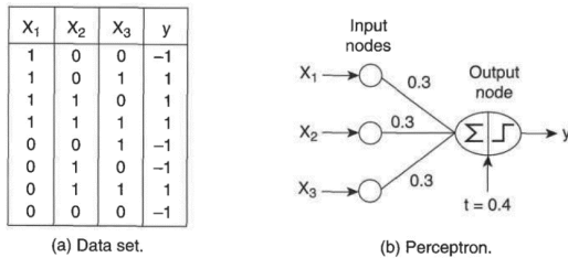
Figure 5.14. Modeling a boolean function using a perceptron.
