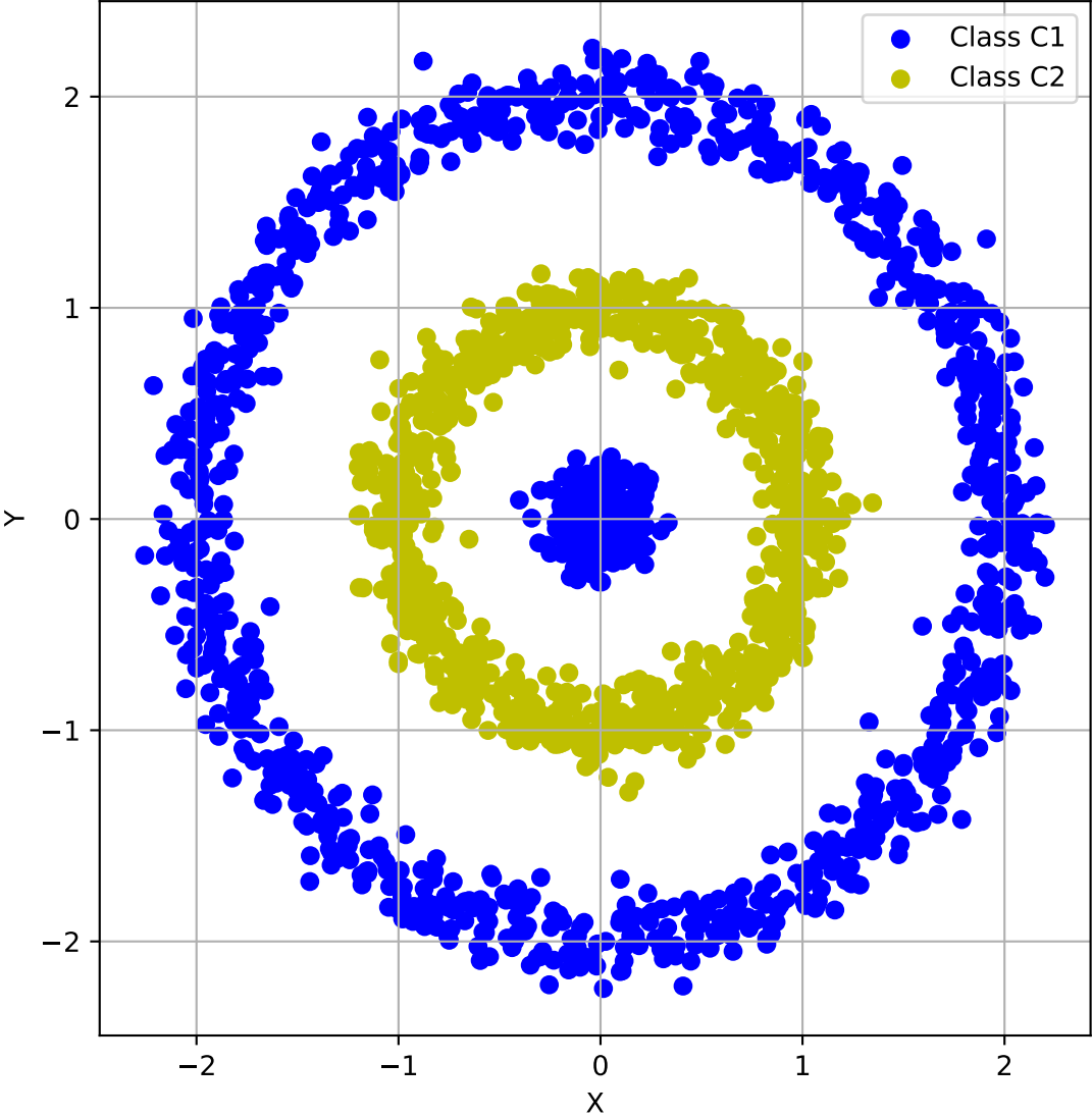
Scatter Plot of Circularly Distributed Data with Gaussian Noise
