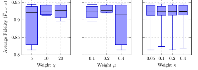
FIG. 11. Sensitivity of the average fidelity at \sigma_{\text{noise}} = 1 MHz to the UFO weights, shown separately for the fidelity weight \chi , the boundary weight \mu and the runtime weight \kappa . Underweighting fidelity ( \chi = 5 ) opens a failure mode near \bar{F} \approx 0.82 ; \mu = 0.4 is strongly bimodal; \kappa has almost no effect in this fixed-horizon regime.
