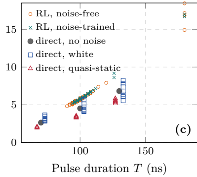
Quasi-static excess infidelity ( 10^{-3} )
