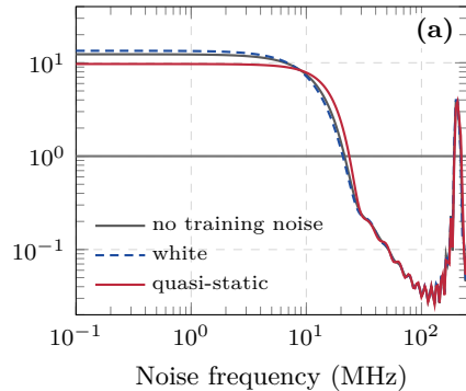
Normalized filter function
