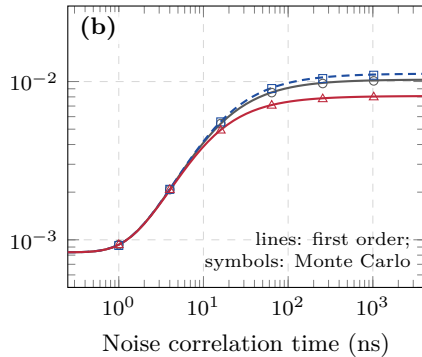
Excess infidelity at 0.2 MHz
