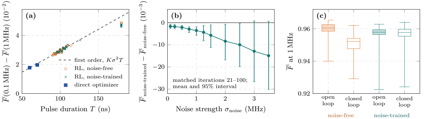
FIG. 2. Open-loop robustness and stochastic training. (a) Excess infidelity at 1 MHz against pulse duration for all pulses of a matched pair of RL agents and for the pulses of the direct optimizer, with the first-order prediction of Eq. (18) (dashed); the pulses at 180 ns are rollouts that reached the episode ceiling, where higher orders begin to matter. (b) Paired difference in average fidelity between the noise-trained and the noise-free pulse of the same iteration, for the first matched pair over iterations 21–100, with 95% block-bootstrap intervals; negative values favour the noise-free agent. (c) Average fidelity at 1 MHz of the same checkpoints, replayed open loop (filled) and acting in closed loop on the noisy propagator (open); boxes span the quartiles and whiskers the full range.
