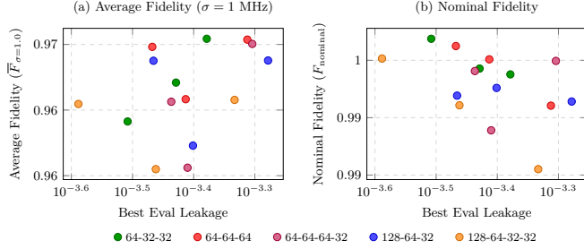
FIG. 10. Architecture trade-offs: evaluation leakage against (a) average fidelity at \sigma_{\text{noise}} = 1 MHz and (b) nominal fidelity. Leakage minimization is not a proxy for robustness — the layout with the lowest leakage, (128, 64, 32, 32), has the worst aggregate cost and the weakest robustness.
