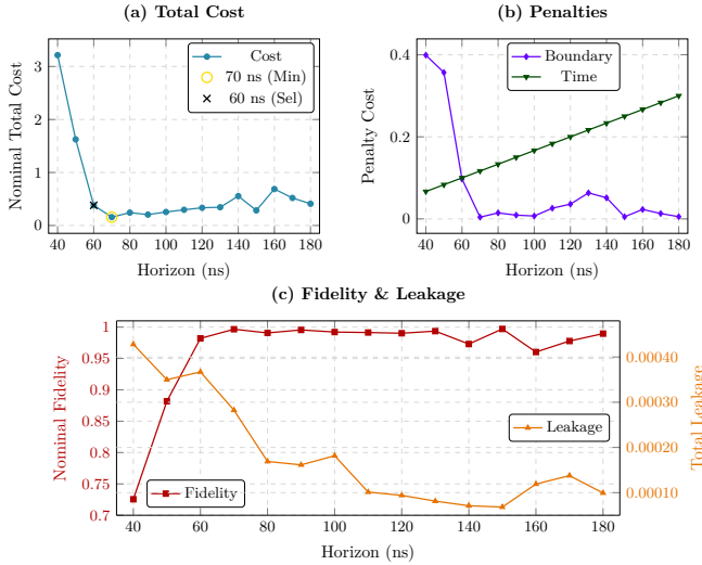
FIG. 3. Adam baseline on N(2.2, 2.2, \pi/2) versus gate horizon. (a) Nominal total cost, with the optimum at 70 ns and the plan selected by the noisy objective at 60 ns both marked. (b) Boundary and runtime penalties. (c) Nominal fidelity and total leakage. The optimum arises from the simultaneous collapse of the boundary term and the rise in fidelity; longer horizons saturate in fidelity and are penalized by runtime.
