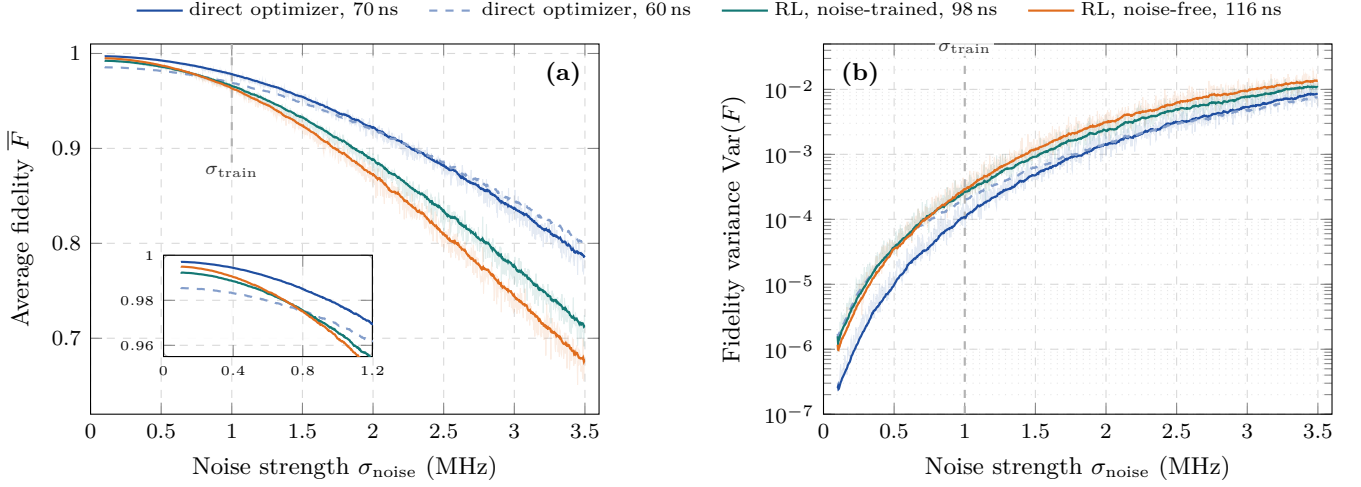
FIG. 1. Robustness on N(2.2, 2.2, \pi/2) of the pulses of Table I and of a shorter, 60 ns pulse from the direct optimizer, replayed open loop. (a) Average fidelity \bar{F}(\sigma_{\text{noise}}) , with the low-noise regime magnified in the inset. (b) Fidelity variance \text{Var}(F) on a logarithmic axis. Lines are exponentially weighted moving averages along the noise axis (spans 50 and 80); the underlying Monte Carlo scatter is shown for three of the curves. The dashed vertical lines mark the training noise \sigma_{\text{train}} = 1 MHz. The 70 ns pulse of the direct optimizer is more robust than both RL pulses at every noise strength, and at high noise the four pulses rank by duration.
