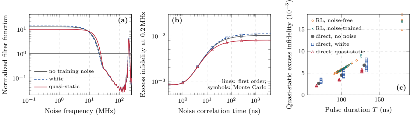
FIG. 3. Noise with memory. (a) Filter functions, summed over the channels and normalized to their average over the Nyquist band, of three 70 ns pulses of the direct optimizer for N(2.2, 2.2, \pi/2) : optimized without noise, under white noise (1 MHz) and under quasi-static noise (0.3 MHz). The average is the same for the three (horizontal line); the low-frequency plateau is not. The peak at 200 MHz is the transition to the leakage levels. (b) Excess infidelity of the same pulses under exponentially correlated noise of standard deviation 0.2 MHz against its correlation time: first-order prediction of Eq. (A2) (lines) and Monte Carlo replay (8000 realizations, symbols). (c) Excess infidelity under quasi-static noise of 0.1 MHz against duration, for the pulses of the first matched pair of RL agents and for pulses of the direct optimizer optimized at 70, 100 and 130 ns under the three noise models (eight seeds for each stochastic model; the white and quasi-static symbols are shifted by \pm 3 ns for visibility).
