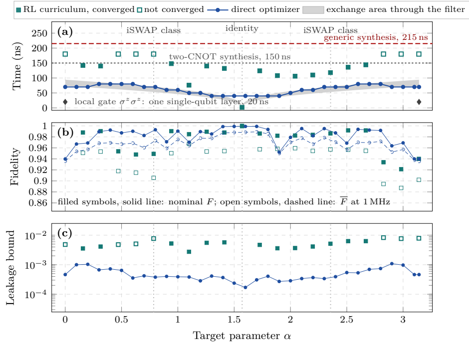
FIG. 4. Runtime across N(\alpha, \alpha, \pi/2) . (a) Final evaluation runtime of the RL curriculum (filled squares: converged; open squares: not converged, the rollout running to the 180 ns ceiling) and horizon selected by the direct optimizer (circles). Grey band: shortest time in which the coupling can deliver the exchange area 2|\alpha - \pi/2| through the bandwidth filter under the 20 MHz bound, without (lower edge) and with (upper edge) the condition that it returns to zero at the end of the pulse (Sec. VI E). Dashed: generic synthesis reference of Ref. [4], 215 ns; dotted: two-CNOT synthesis, Eq. (20), 150 ns; diamonds: the local members \sigma_1^z \sigma_2^z , one layer of single-qubit gates. Vertical lines mark the identity target \alpha = \pi/2 and the iSWAP-equivalent targets |\alpha - \pi/2| = \pi/4 . (b) Nominal fidelity (filled symbols, solid line) and average fidelity at \sigma_{\text{noise}} = 1 MHz (open symbols, dashed line) for both sweeps; the cold-start curriculum point \alpha = 0 (0.56 and 0.61) is off scale. (c) Leakage bound of the evaluated pulses, with the symbols of panel (a).
