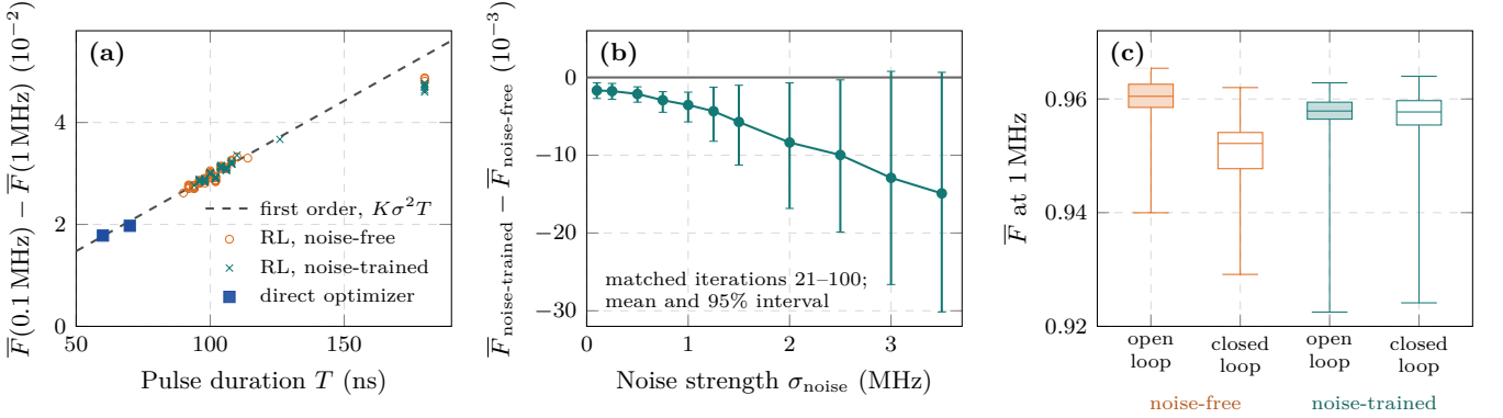
FIG. 2. Open-loop robustness and stochastic training. (a) Excess infidelity at 1 MHz against pulse duration for all pulses of a matched pair of RL agents and for the pulses of the direct optimizer, with the first-order prediction of Eq. (18) (dashed); the pulses at 180 ns are rollouts that reached the episode ceiling, where higher orders begin to matter. (b) Paired difference in average fidelity between the noise-trained and the noise-free pulse of the same iteration, for the first matched pair over iterations 21–100, with 95% block-bootstrap intervals; negative values favour the noise-free agent. (c) Average fidelity at 1 MHz of the same checkpoints, replayed open loop (filled) and acting in closed loop on the noisy propagator (open); boxes span the quartiles and whiskers the full range.
