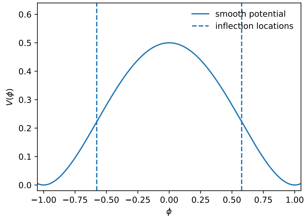
(a) Smooth double well
