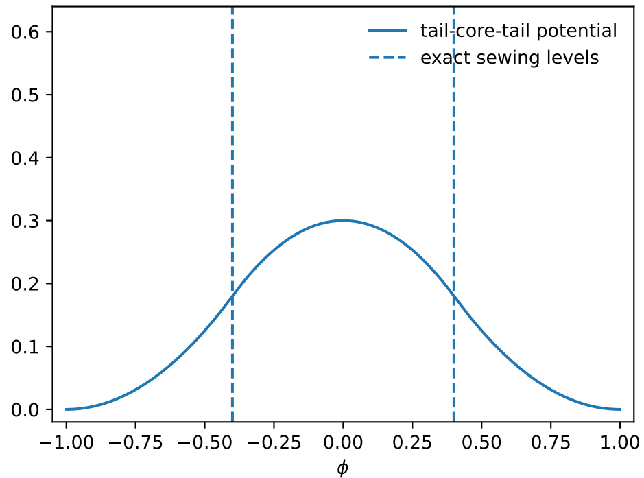
(b) Piecewise model
