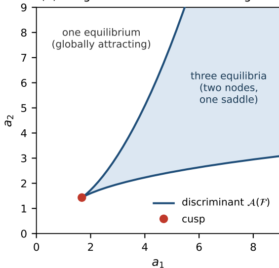
(b) image under \mathcal{A} : bifurcation diagram
