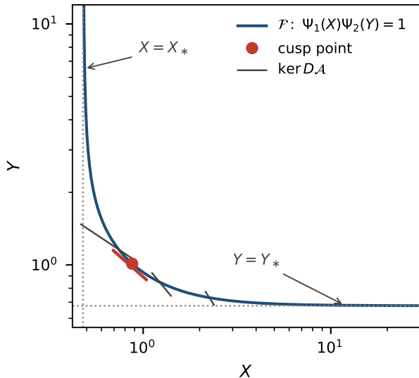
(a) singular set of \mathcal{A} in the state plane
