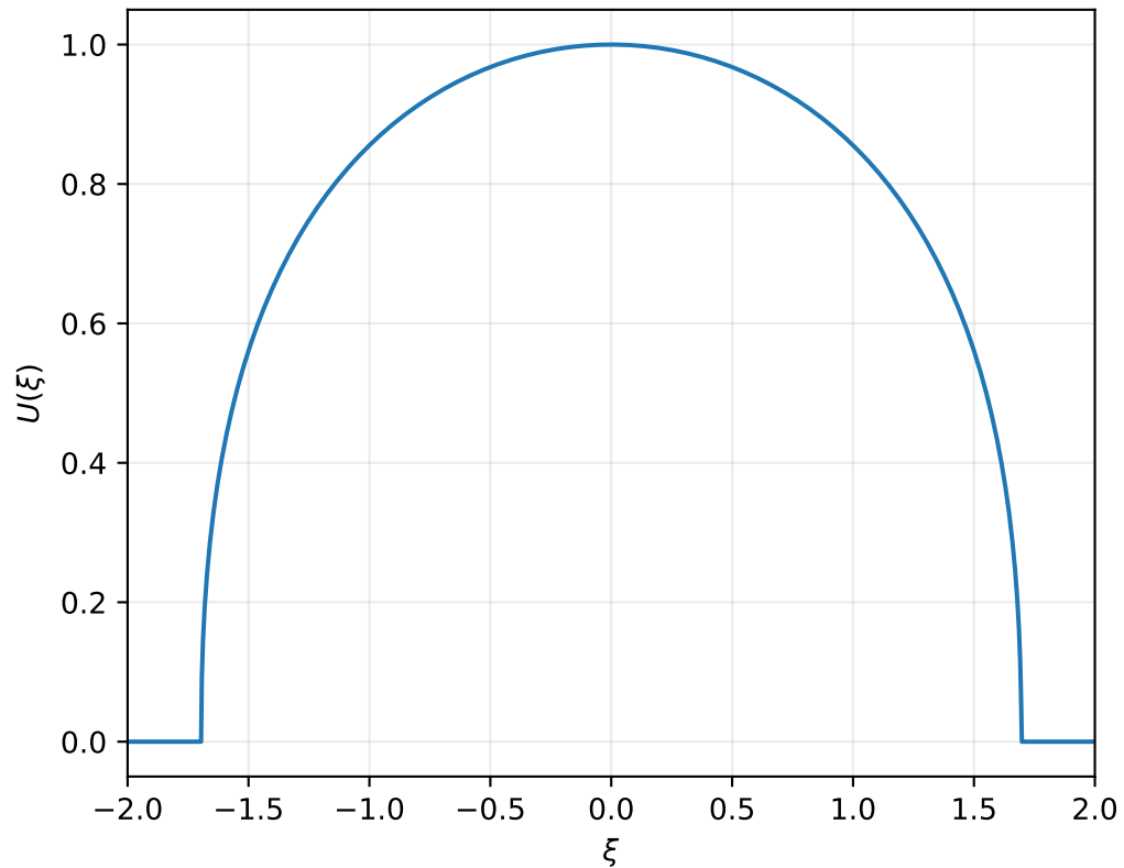
Regularity-threshold compacton: a = 3 , b = 2 , E = -1
